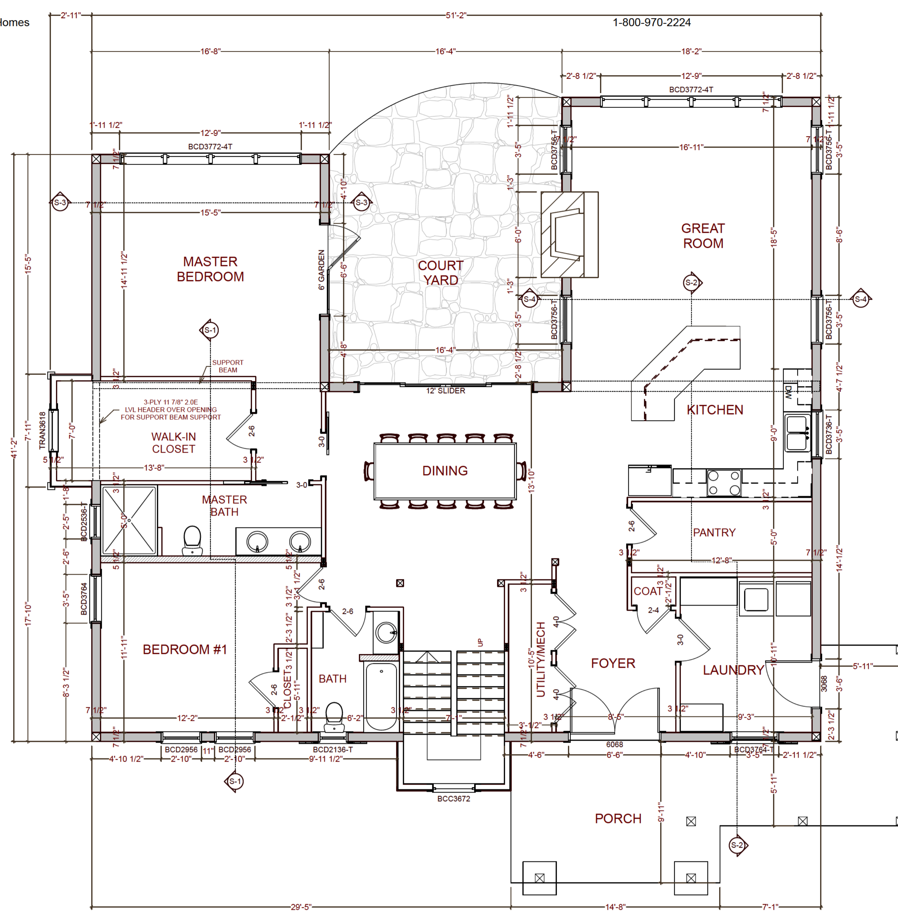
MAIN FLOOR PLAN
