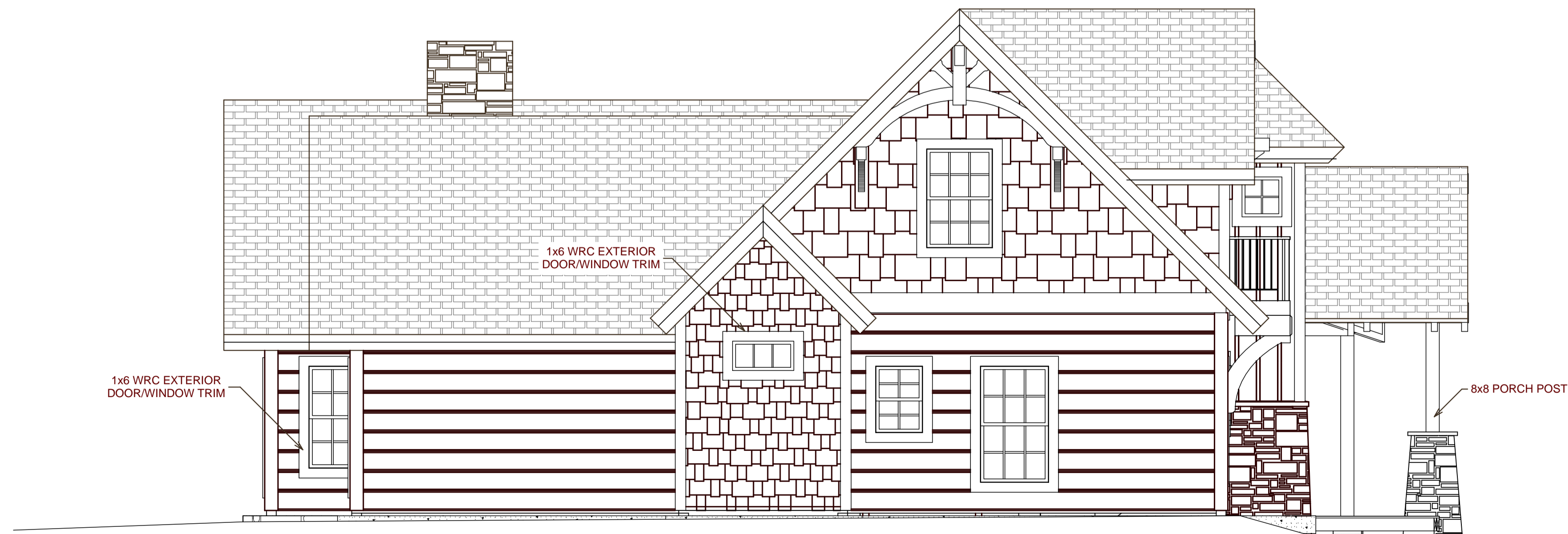
LEFT ELEVATION
