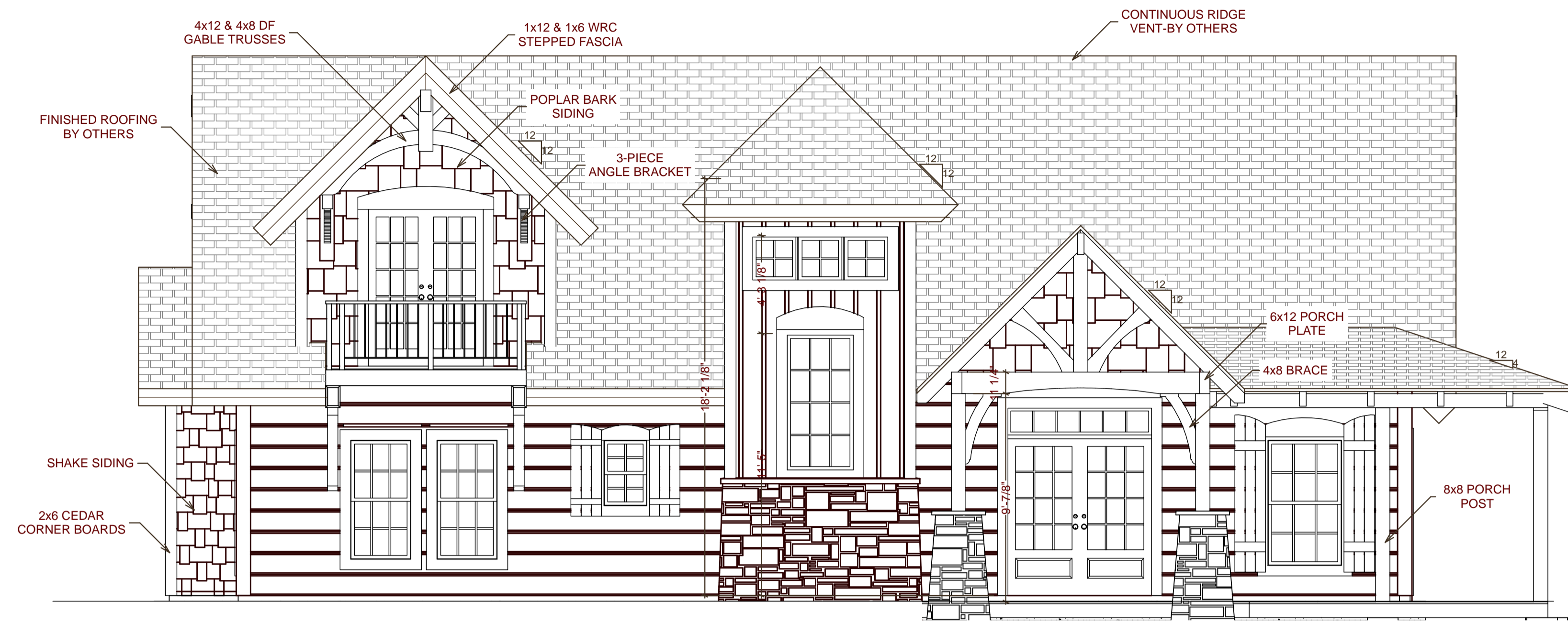
FRONT ELEVATION
