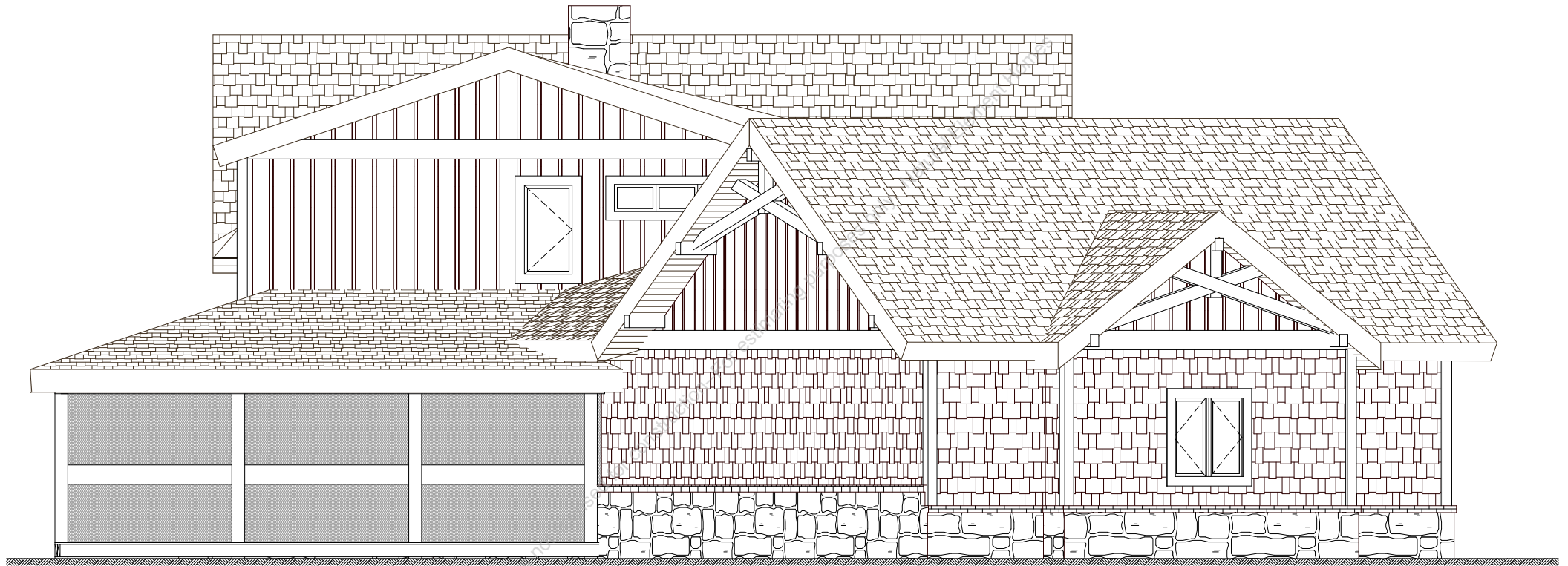
LEFT ELEVATION
