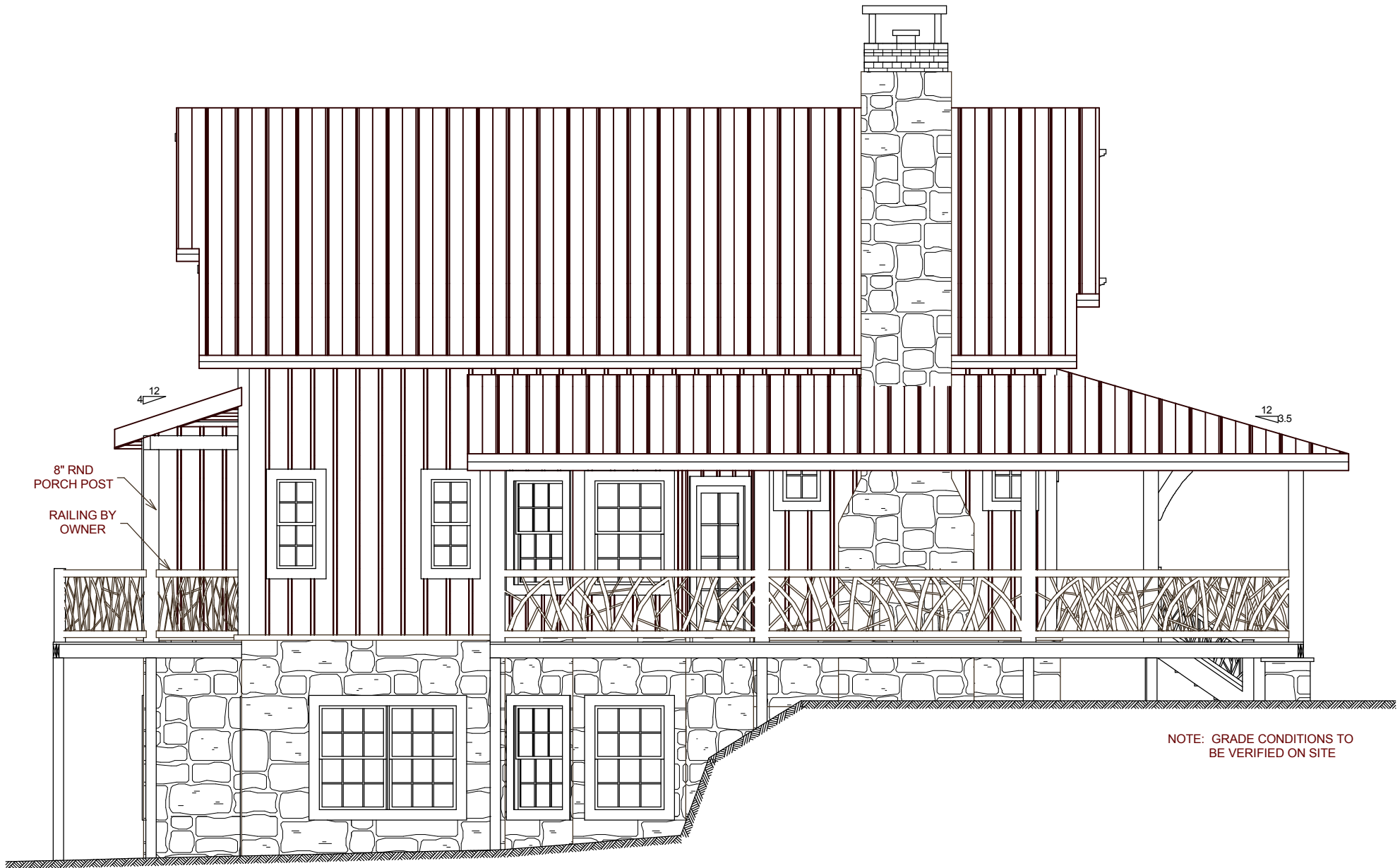
LEFT ELEVATION
